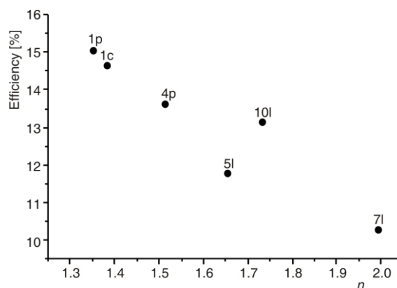
Figure 1. Dependence of efficiency on the ideality factor
