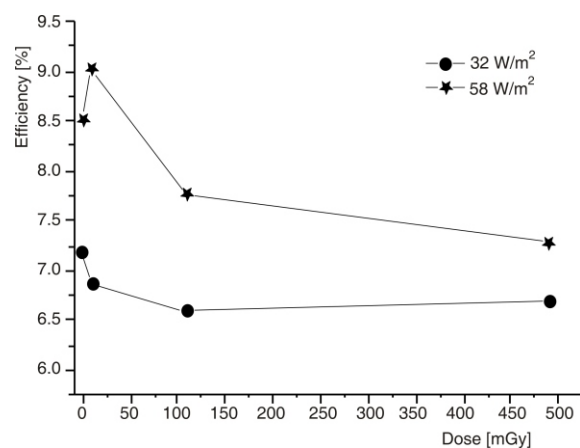
Figure 4. Dependence of efficiency on doses (gamma irradiation)
