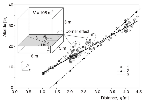
Figure 7. Albedo dependence vs. distance r . Ignalina NPP case with point source: (1) simulation data, (2) according to formula (4), and (3) according to formula (5)
