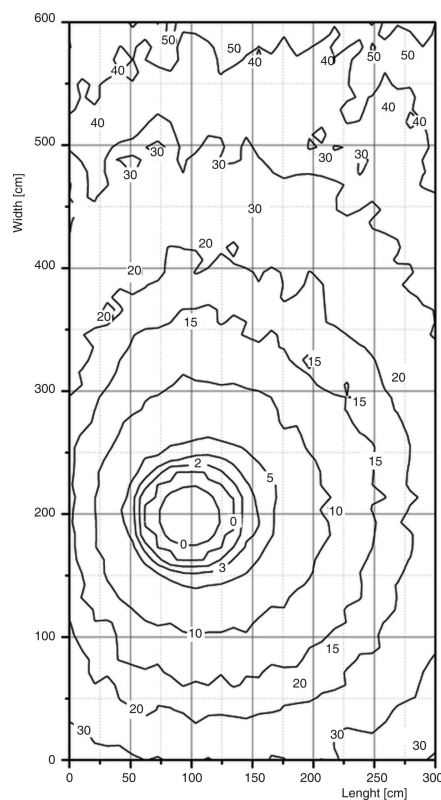
Figure 10. Dose rate map of secondary radiation (in %): real case of Ignalina NP
