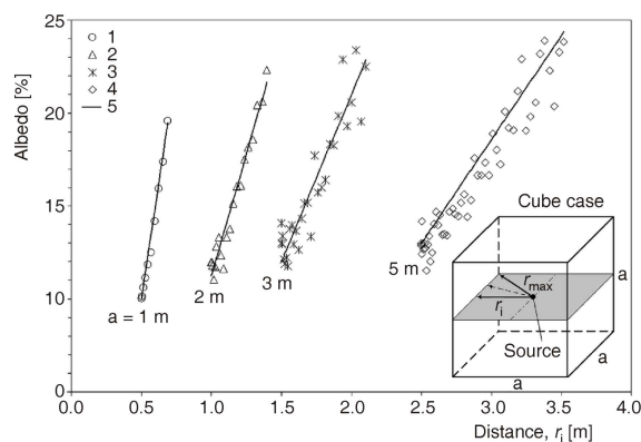
Figure 6. Albedo dependence vs. distance r . Cube case: (1) volume 1 m 3 ; (2) 8 m 3 ; (3) 27 m 3 ; (4) 125 m 3 ; and (5) according formula (4)
